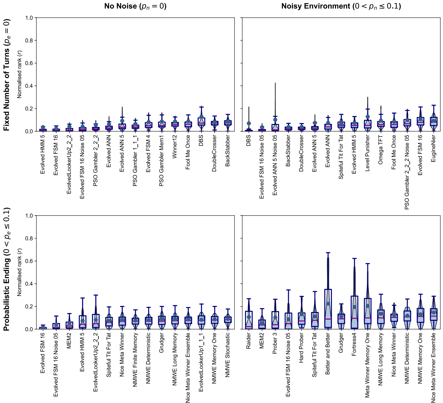
Fig 3. r distributions of the top 15 strategies in different environments. A lower value of \bar{r} corresponds to a more successful performance. A strategy's r distribution skewed towards zero indicates that the strategy ranked highly in most tournaments it participated in. Most distributions are skewed towards zero.
