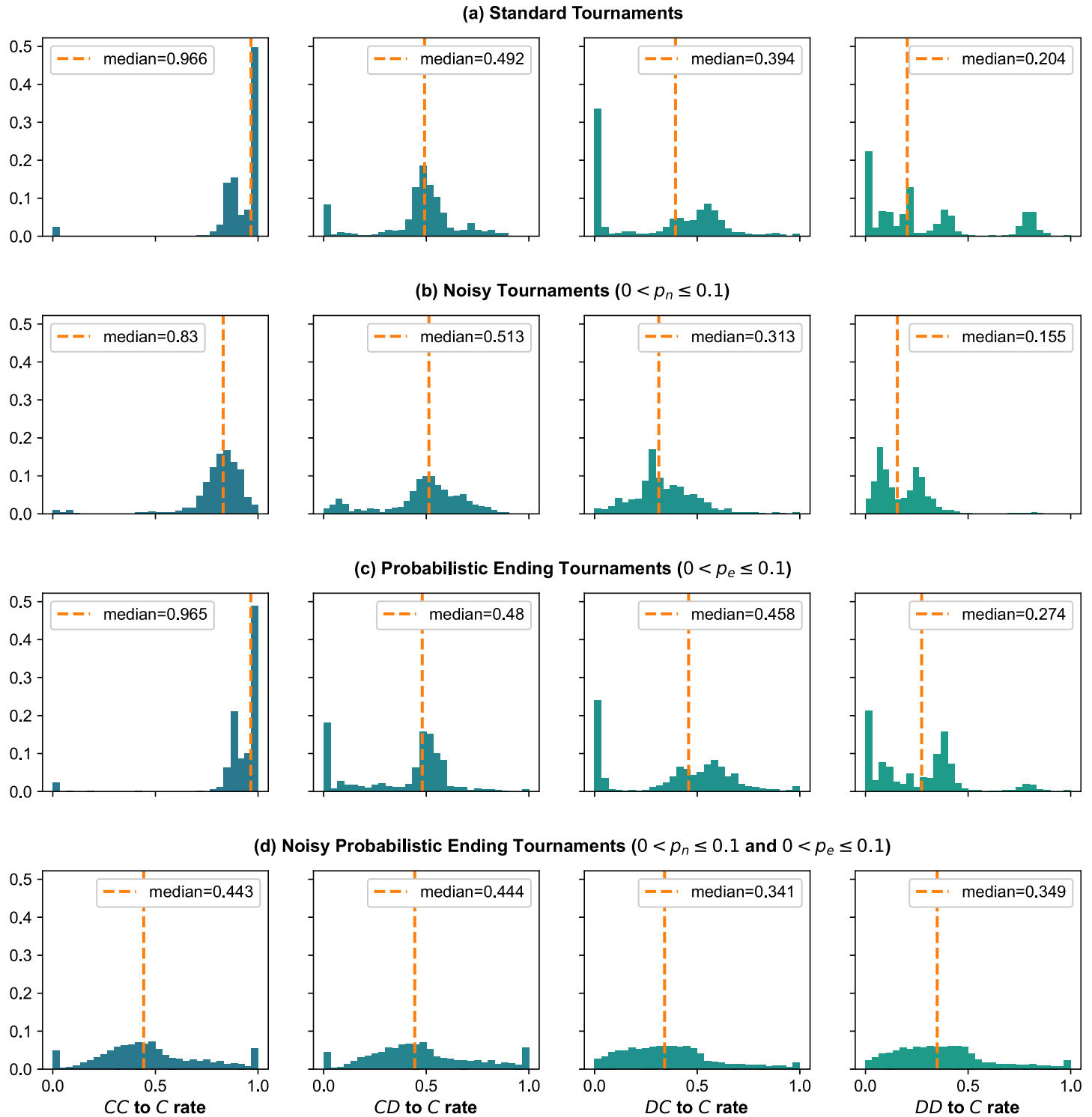
Fig 6. Distributions of rates CC to C, CD to C, DC to C, and DD to C for the winners of tournaments. The result summary from the tournaments records how often each strategy cooperated after each possible outcome of the previous round. Specifically, we analyze the probability with which a strategy chose C following the outcomes. Here, we plot the distributions of these probabilities for the winners of the tournaments. We separate them by type of tournament, from top to bottom: standard, noisy, probabilistic ending, and noisy probabilistic ending. From left to right, we plot the distributions of cooperation after the outcomes CC, CD, DC, and DD.
