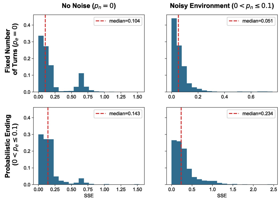
Fig 5. Distributions of SSE error for the winners of tournaments. Here, we again consider the winners of the tournaments, separated by type of tournament, and plot their SSE error. As a reminder, the SSE error indicates how closely a strategy behaves like a Zero-Determinant (ZD) strategy, and subsequently, in an extortionate way. An SSE value of 1 indicates no extortionate behavior at all, whereas a value of 0 indicates that a strategy is behaving as a ZD.
