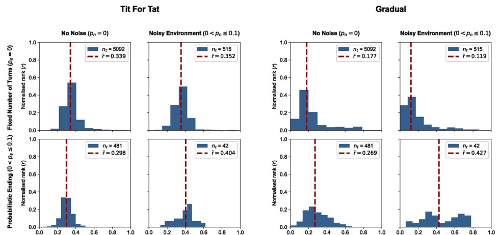
Fig 2. Examples of normalized rank distributions for two strategies, TFT and Gradual. We plot the distributions of r for the two strategies in the four tournament types. As a reminder, lower values of r correspond to better performances. The top left quadrant of each plot shows the distribution for standard tournaments (fixed number of turns and no noise). The top right quadrant shows the distribution for noisy tournaments (fixed number of turns and noise). The bottom left quadrant shows the distribution for probabilistic ending tournaments (no noise and probabilistic ending). Finally, the bottom right quadrant shows the distribution for noisy probabilistic ending tournaments (noise and probabilistic ending). In each quadrant, we also show the number of data points. Both strategies participated in a similar number of tournaments. Based on the median rank, which we use in this work to define overall performance, TFT performs best in probabilistic ending tournaments, whereas Gradual was in standard tournaments.
