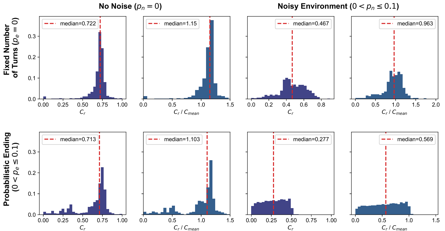
Fig 4. Distributions of C_r and C_r/C_{\text{mean}} for the winners of tournaments. In this distribution, we consider the winners of the tournaments, specifically the strategies that ranked first in each tournament. For each type of tournament, we plot the cooperation rate of the winner in the tournament they won, as well as the ratio of the winner's cooperation rate to that of the entire tournament. A value of C_r/C_{\text{mean}} = 1 implies that the cooperation ratio of the winner was the same as the mean cooperation ratio of the tournament.
